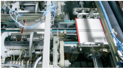
Side folding station
