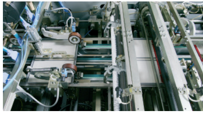
Head/Tail folding and corner tucking station
