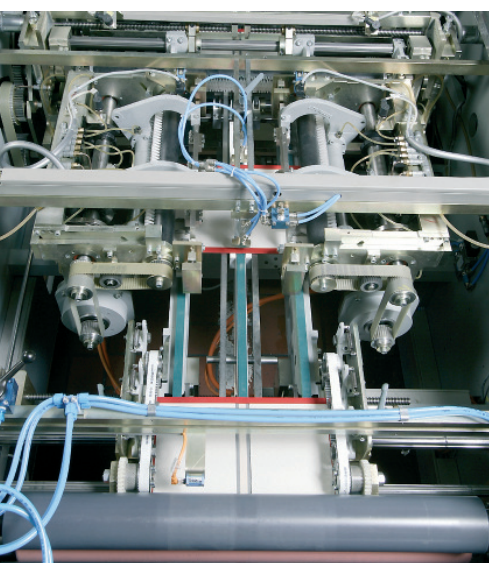
Working process always visible to operator
