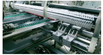
Folding stations with brushes for superior case quality
