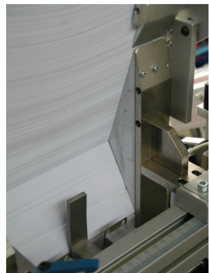
Tapered construction for additional discharge of the product stack.
